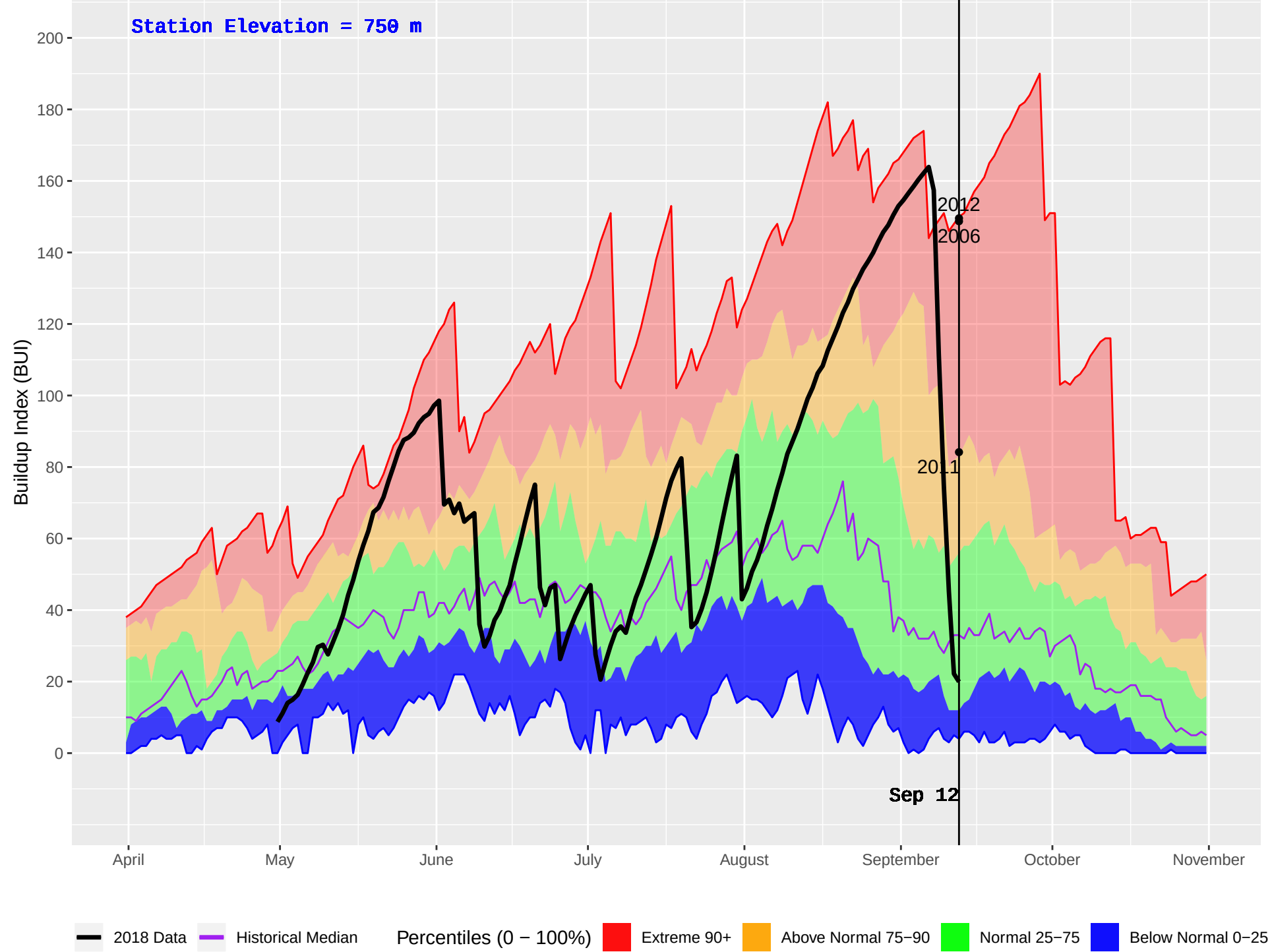
FORT ST JAMES (146) : Historical (1979–2016) and Current (2018) Daily Buildup Index (BUI)
