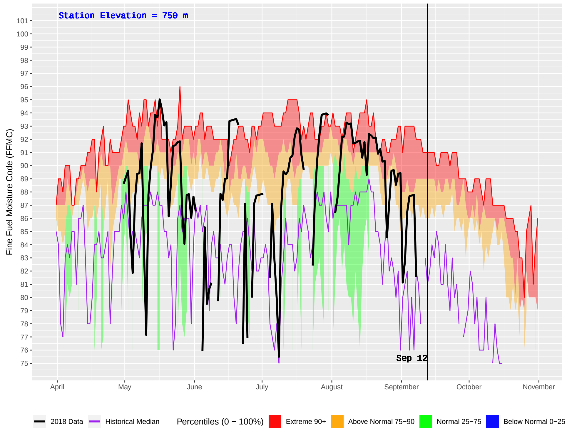
FORT ST JAMES (146) : Historical (1979–2016) and Current (2018) Daily Fine Fuel Moisture Code (FFMC)
