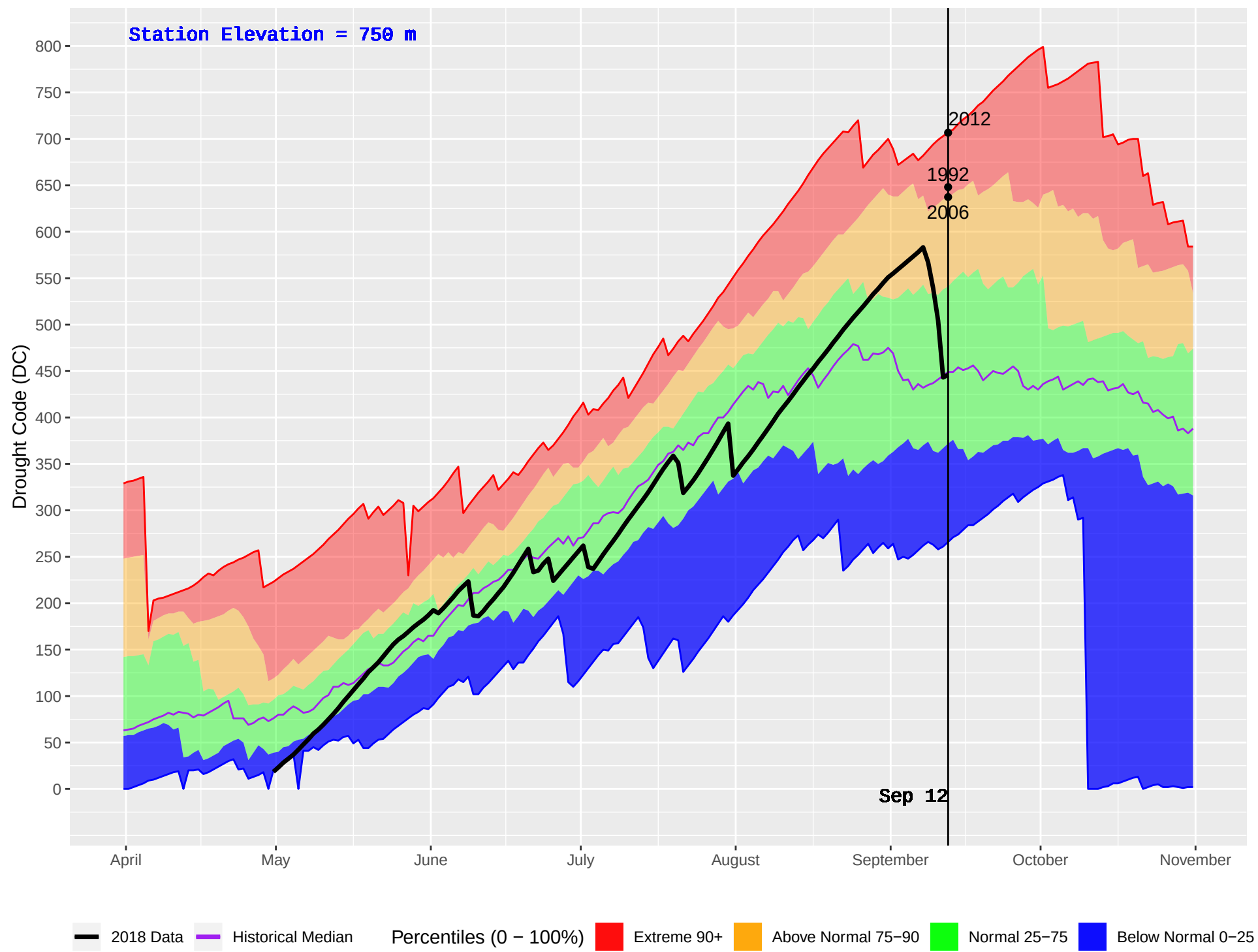
FORT ST JAMES (146) : Historical (1979–2016) and Current (2018) Daily Drought Code (DC)
