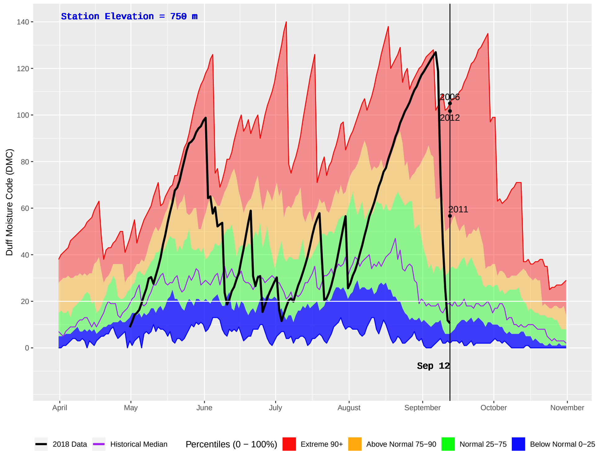
FORT ST JAMES (146) : Historical (1979–2016) and Current (2018) Daily Duff Moisture Code (DMC)
