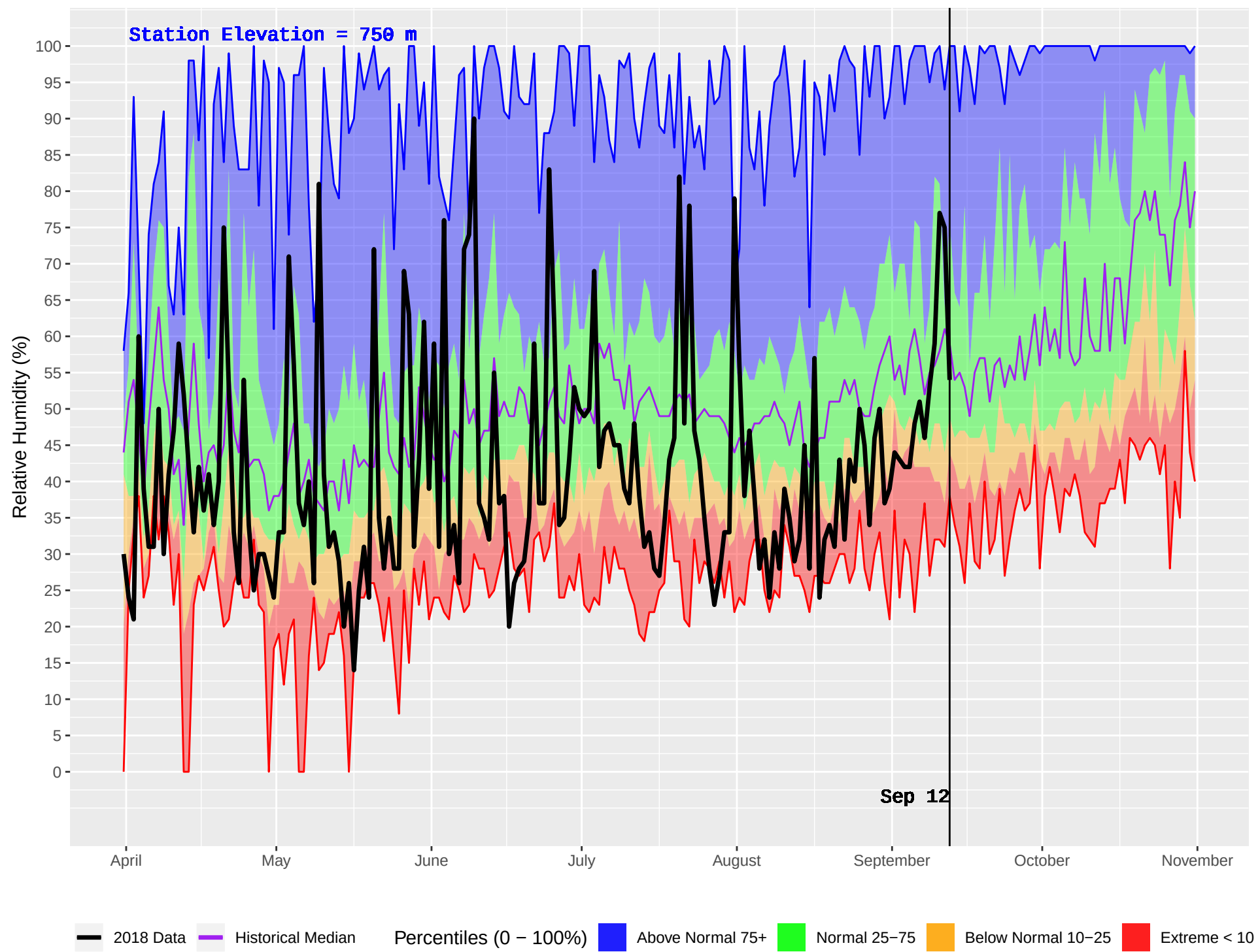
FORT ST JAMES (146) : Historical (1979–2016) and Current (2018) Daily Relative Humidity
